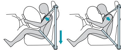
A Pre-Tensioner automatically retracts the seatbelt and helps secure the occupant at the moment of severe forward deceleration. If the shoulder belt forces applied to the occupant reaches a predetermined amount, then the Force Limiter allows the webbing to extend to help reduce pressure on the occupant's chest.
